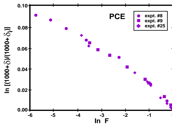
Figure 1. Abiotic Oxidation of PCE (Poulson and Naroaka, 2002)
